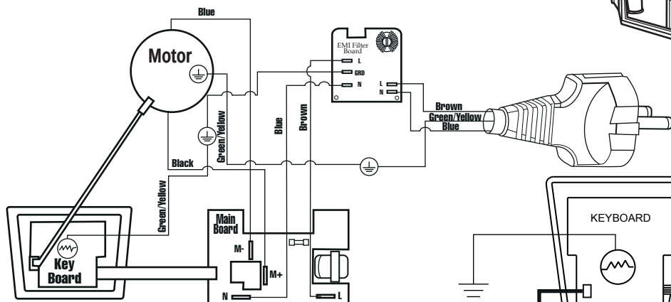
Wiring Diagram
