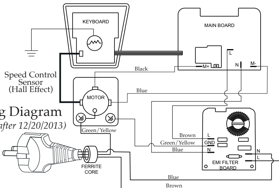
Wiring Diagram
