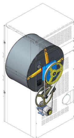
TRASMISSIONE TRANSMISSION
